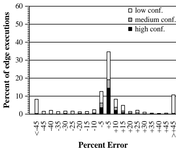
Figure 9: Distribution of Errors in Edge Frequencies (Weighted by Edge Executions)
