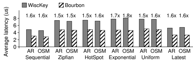
Figure 11: Request Distributions. The figure shows the average lookup latencies of different request distributions from AR and OSM datasets.
